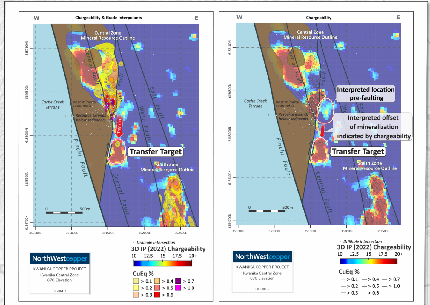
Figure Note: Level plans approximately 200m below surface at 870m above sea level. (Left) highlights the Transfer Target chargeability anomaly (block model) with property scale structural interpretation, and grade shell interpolations (colored polygons) from leapfrog geo at the Central and South Zone. (Right) shows the same level plan highlighting the potential position of the Transfer Target relative to the Central Zone mineralization pre-faulting.
