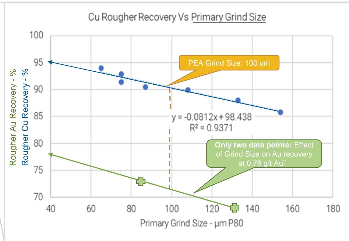
Figure 13-4: Primary Grind Size vs Copper Recovery
