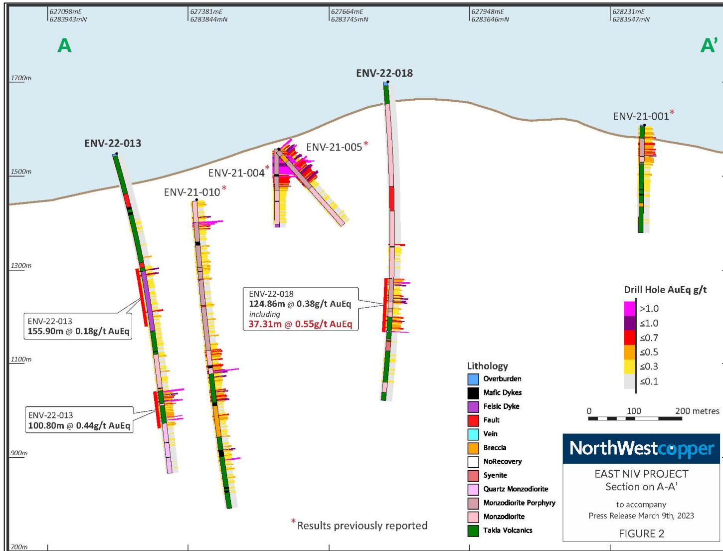
Figure 2: A-A' Cross Section
