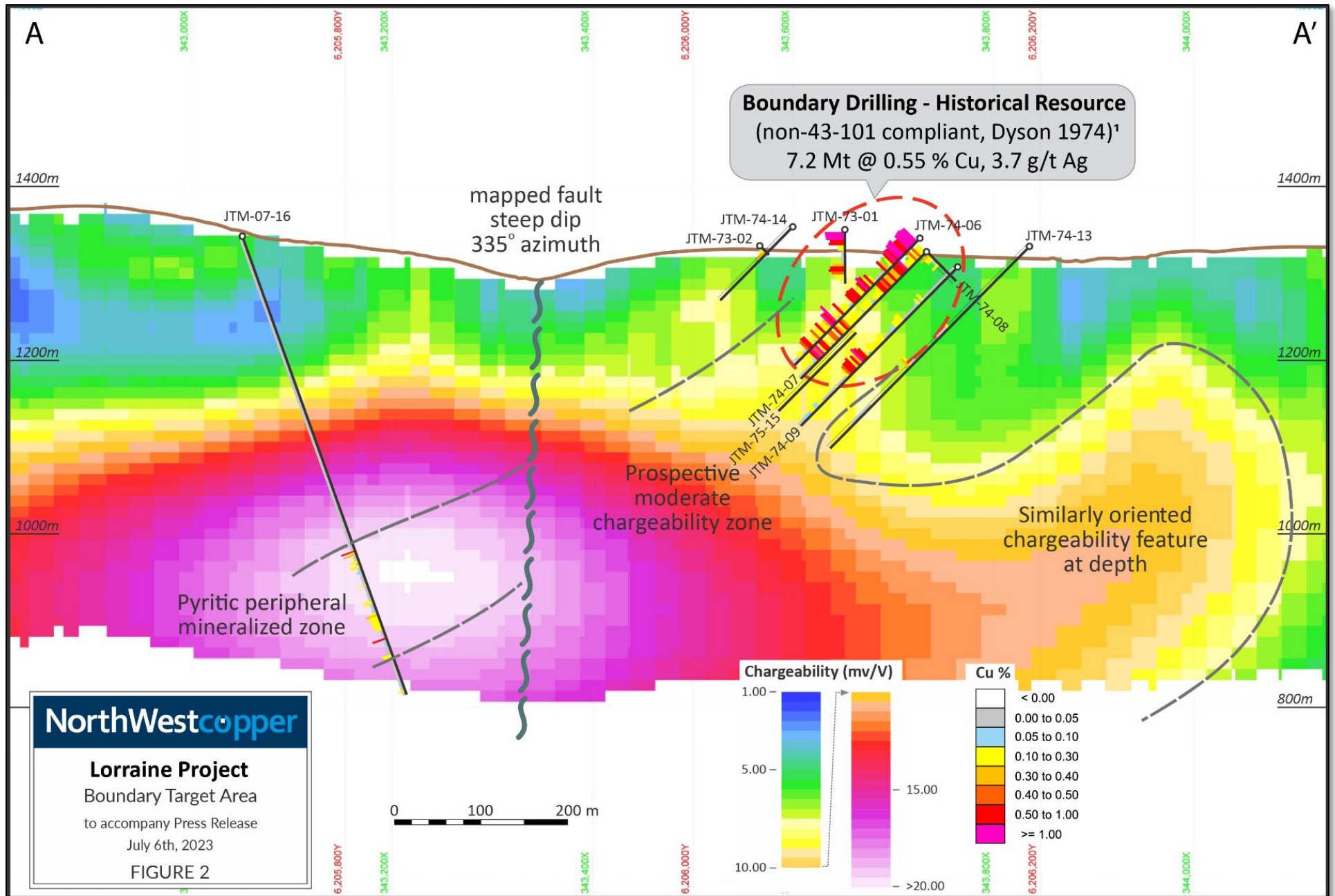
Figure 2. Cross Section A-A' Showing Chargeability Model and Historic Drilling
