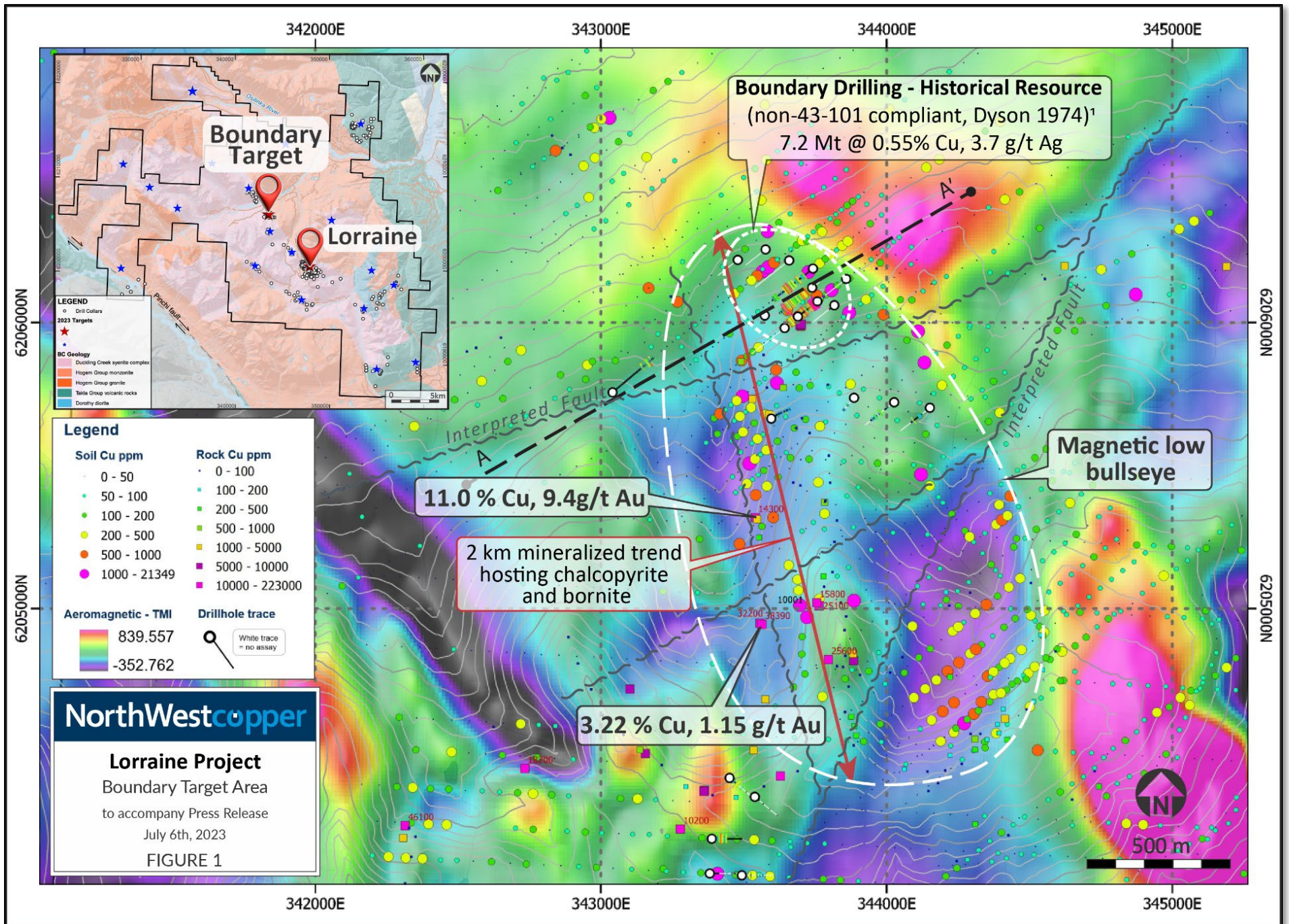
Figure 1. Plan View of the Boundary Target Area
